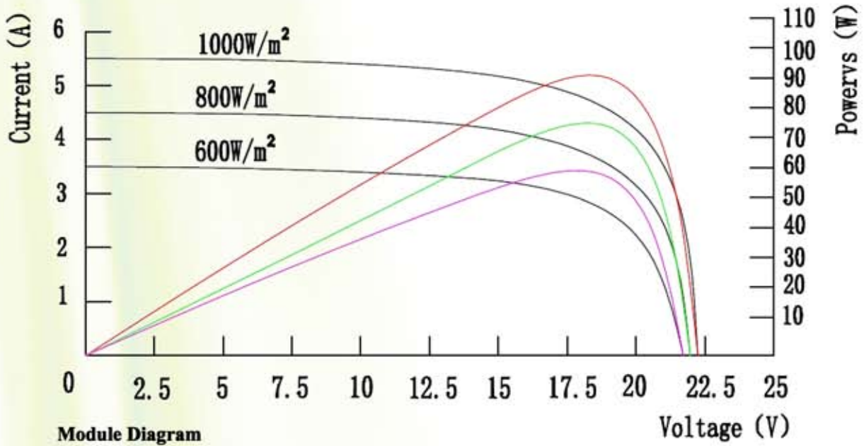
The I-V, Powers curve of 95W monocrystalline module
