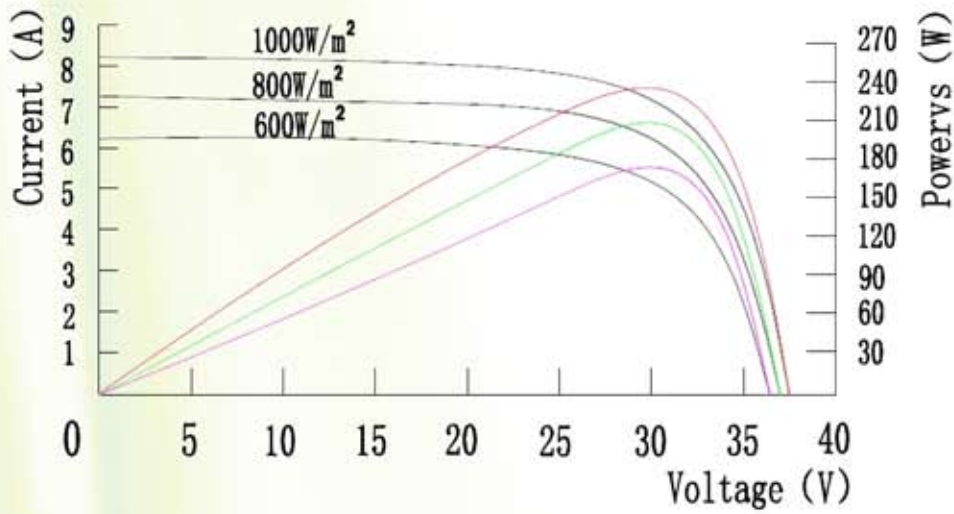
The I-V, Powers curve of 230W multicrystalline module
