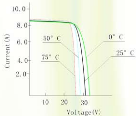
I-V curve
