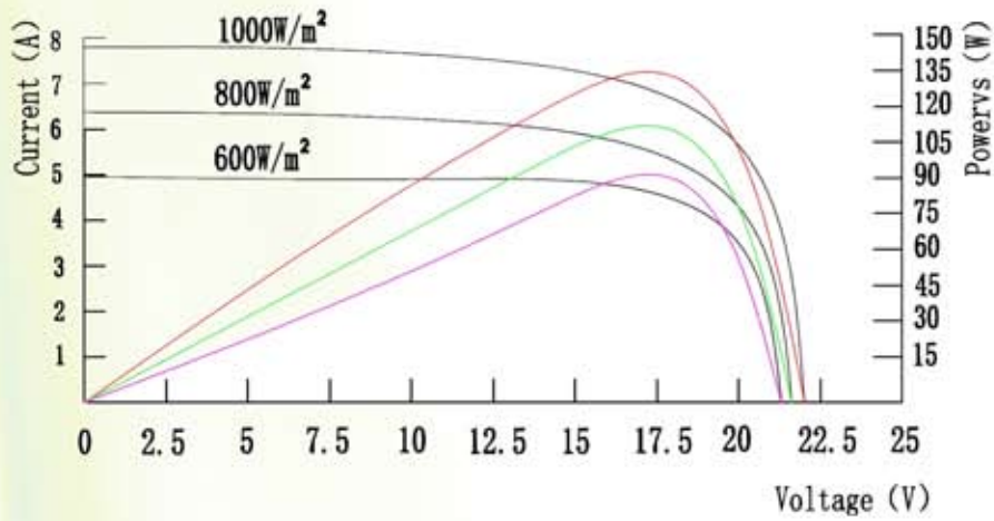
The I-V, Powers curve of 135W multicrystalline module
