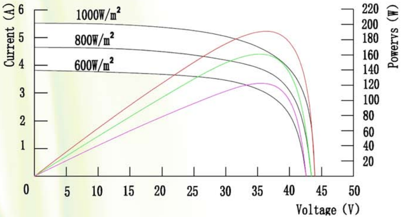
The I-V, Power curve of 190W monocrystalline module
